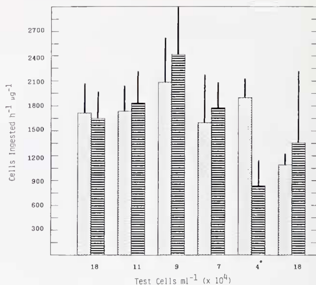
Figure 1. The influence of algal cell concentration ( Isochrysis sp., Tahitian isolate) on weight-specific ingestion rate of juvenile Crepidula formicata . One group of 12 juveniles (dotted bars) was fed at an initial cell concentration of 18 \times 10^4 cells \text{ml}^{-1} in each 1-h feeding bout. The other group of 12 juveniles (striped bars) was fed at progressively lower food concentrations every 1 h as indicated. To complete the experiment (extreme right), both groups of snails were offered 18 \times 10^4 cells \text{ml}^{-1} . *Represents a significant difference between means ( P < 0.05 , one-way analysis of variance). Error bars indicate one standard deviation above the mean.
